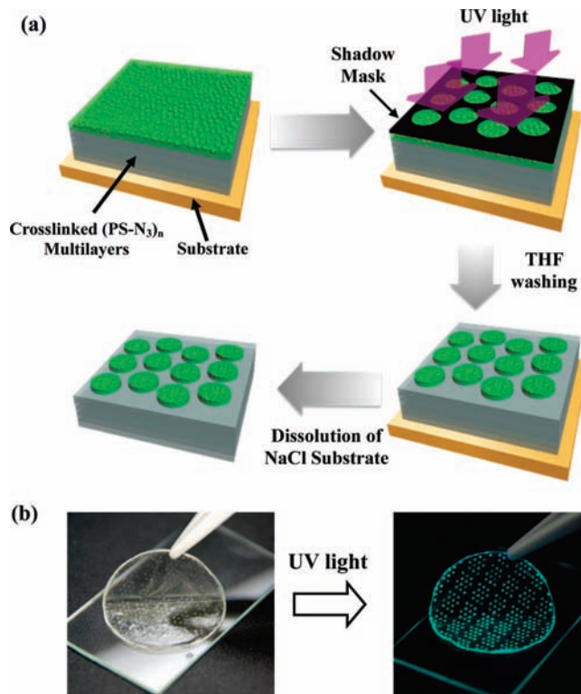
Figure 6. (a) Schematic for the preparation of patterned free-standing multilayer films. (b) Photographic images of \text{PS}-\text{N}_3-\text{SH} -green QD layer patterned onto (\text{PS}-\text{N}_3)_{40} multilayer film. In this case, the size of the patterned dot is about 500 \mu\text{m} .
