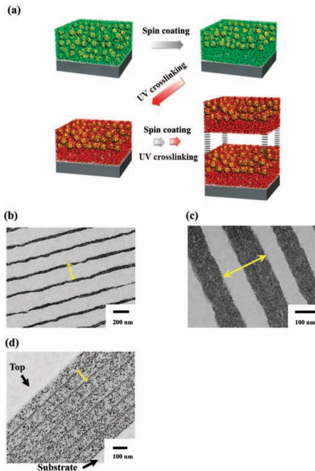
Figure 5. (a) Schematic for the buildup of (\text{PS}-\text{N}_3-\text{SH}-\text{QDs}:\text{PS}-\text{N}_3)_n multilayers. Cross-sectional TEM images of (b) (\text{PS}-\text{N}_3-\text{SH}-\text{QDs}:\text{PS}-\text{N}_3)_{28} , (c) (\text{PS}-\text{N}_3-\text{SH}-\text{QDs})_{10} multilayers containing excess \text{PS}-\text{N}_3-\text{SH} and (d) (\text{PS}-\text{N}_3-\text{SH}-\text{QDs})_7 multilayers without excess \text{PS}-\text{N}_3-\text{SH} . As indicated by arrows, the single layer thicknesses of (\text{PS}-\text{N}_3-\text{SH}-\text{QDs}:\text{PS}-\text{N}_3)_{28} , (\text{PS}-\text{N}_3-\text{SH}-\text{QDs})_{10} , and (\text{PS}-\text{N}_3-\text{SH}-\text{QDs})_7 multilayers spin-deposited at 3000, 1500, and 1500 rpm are 265, 225, and 127 nm, respectively.
